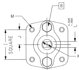
ACTUATOR MOUNTING
